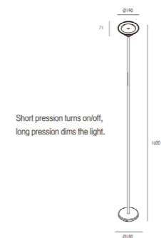
KEBI Floor Lamp (12W)
