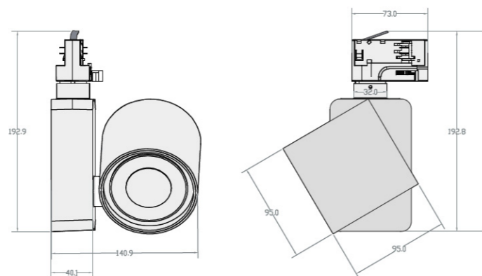
Size diagram
