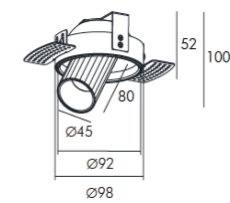
XILE Down light Trim-less
