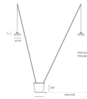
KEBI Floor Lamp (2x10W)
