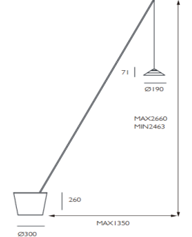
KEBI Floor Lamp (10W)
