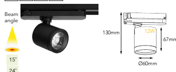
TL6067.12 Lens version
