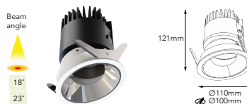
DL110121T.20 Deep antiglare downlight Tiltable
