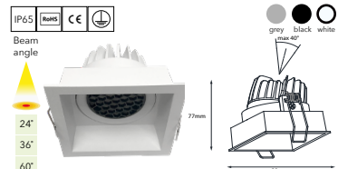
SL9090D.08 Ip65 Cree/Citizen led
