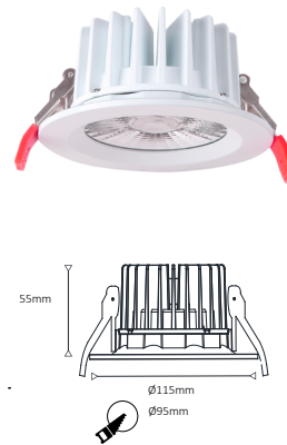
DW11555 15W Ip65 Cree/Citizen led
