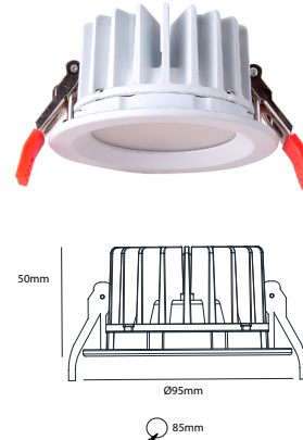
DW9550SMD 10W Ip65 Samsung
